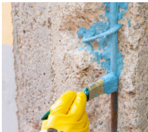
Applying Mapefer 1K Zero
